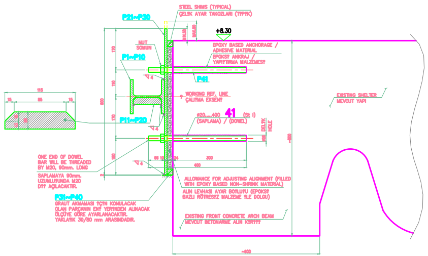
TYPICAL CROSS SECTION TIPIK KESİT SCALE / ÖLÇEK : 1/5
